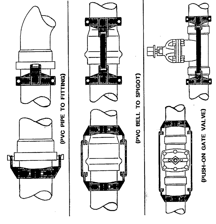
JOINT RESTRAINT
